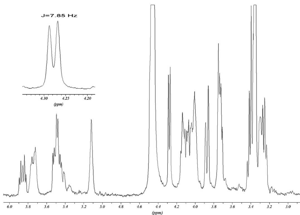
Fig. 3. 1 H-NMR spectrum of GlcCer from C. gloeosporioides . Inset: Anomeric region (H-1) and coupling constant ( J_{1,2} 7.85 Hz).
